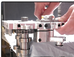
Bolt oil pump to camplate finger tight DO NOT use loctite or hardening compound
