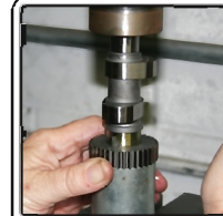
Press cam gears onto camshafts
