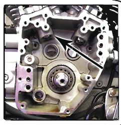
Crank bearing boss & lifter bosses
