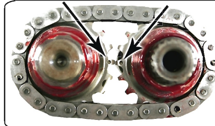
Line up timing marks and pre-lube cam journals
