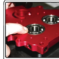
Verify bearings are flush with camplate
