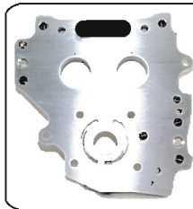
Install block off plates when installing gear drive cams in hydraulic tensioner style camplates
